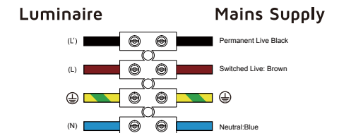
Fig.1 Mains Input Termination
